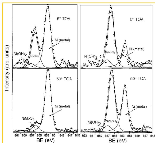
FIGURE 8. Variable-angle Ni2p 3/2 XPS spectra from the passive film formed at -180 mV SCF for 1 h on nitrided and non-nitrided MoNi 4 thin films. All take-off angles measured with respect to the sample surface. Peak identification as shown
