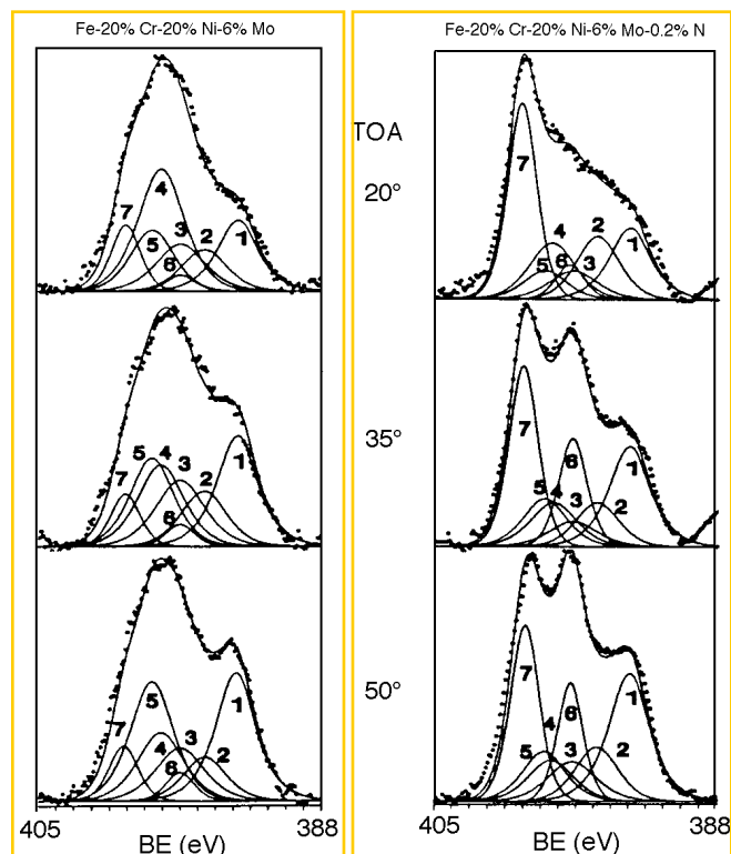
FIGURE 5. N1s and Mo3p XPS spectra for the molybdenum-bearing alloys polarized at -100 \text{ mV}_{\text{SCE}} for 10 min in 0.1 M HCl + 0.4 M NaCl at room temperature. Peak identification for Mo3p 3/2 : (1) Mo 0 ; (2) MoO 2 ; (3) Mo 5+ ; (4) MoO 4 2- ; (5) MoO 3 ; and for N1s: (6) nitride; and (7) NH 3 .
