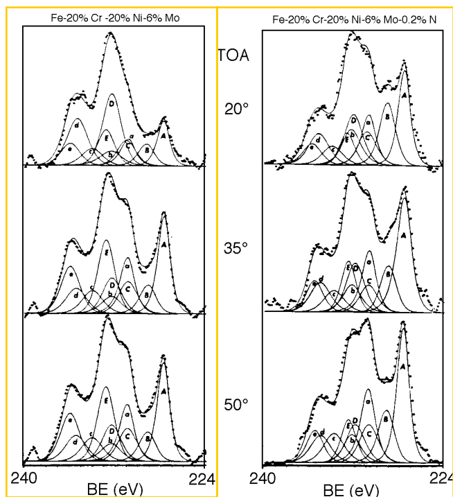
FIGURE 4. Mo3d XPS spectra for the SS polarized at -100 \text{ mV}_{\text{SCE}} for 10 min in 0.1 M HCl + 0.4 M NaCl at room temperature. Peak identification for Mo3d 5/2 : (A) Mo 0 ; (B) MoO 2 ; (C) Mo 5+ ; (D) MoO 4 2- and (E), MoO 3 ; and for Mo3d 3/2 : (a) Mo 0 ; (b) MoO 2 ; (c) Mo 5+ ; (d) MoO 4 2- and (e) MoO 3 .
