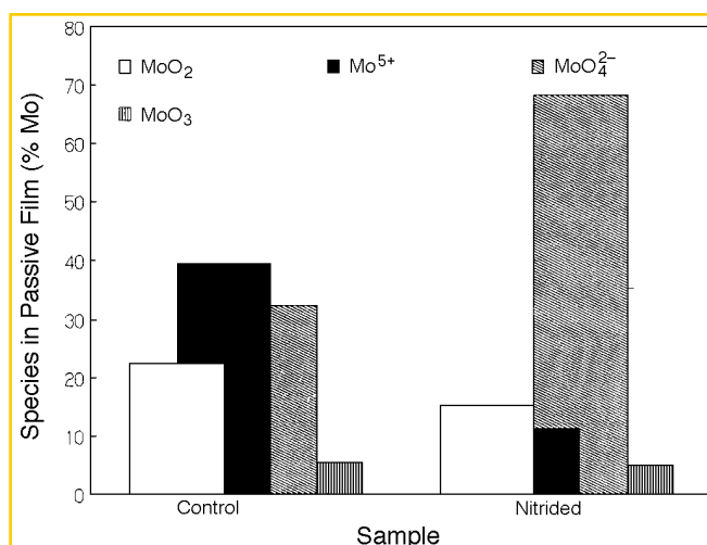
FIGURE 7. Graphical representation of the percentage composition of oxidized molybdenum species in the passive films formed on nitrided and non-nitrided MoNi 4 thin films in 0.1 M HCl at -180 mV SCF for 1 h, derived from XPS data taken with a photoelectron take-off angle of 5°
